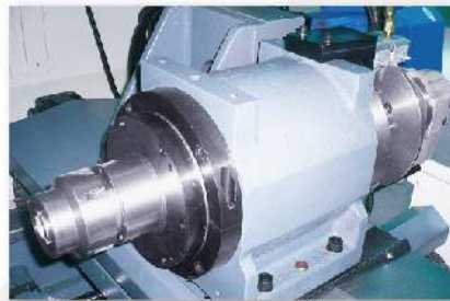
▲ 副主軸C軸功能含碟煞裝置(選配) C-axis function with disk brake device for Sub-spindle(opt)
