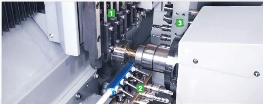
▲ 副主軸C軸功能含碟煞裝置(選配) C-axis function with disk brake device for Sub-spindle(opt)
